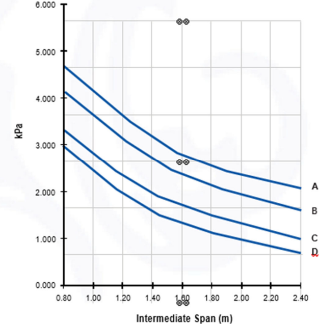
5-Rib 0.55mm
