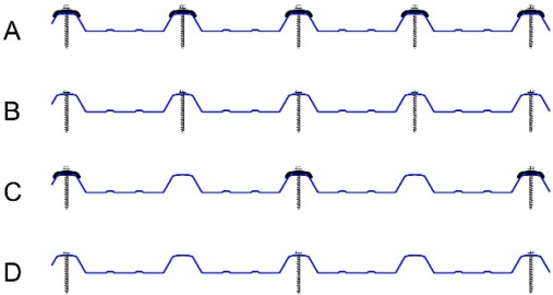
5-Rib 0.40mm
